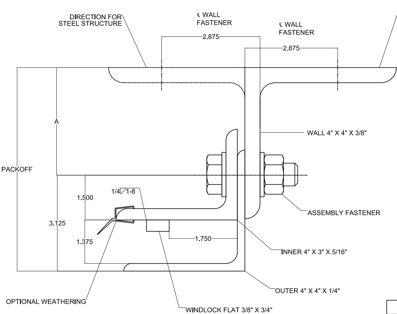
GUIDE ASSEMBLY TYPE 546 SCALE: NTS
