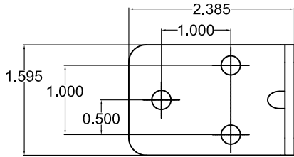
⑧ ENDLOCK / WINDLOCK DETAIL, CP1214 STAMPED STEEL IN ACCORDANCE WITH ASTM A36 OR EQUIVALENT, GALVANIZED IN ACCORDANCE WITH ASTM A123, GRADE 85 ZINC-COATING 1/2 SCALE
