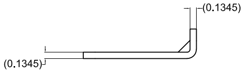
⑨ WINDLOCK DETAIL, CP1513 STAMPED STEEL IN ACCORDANCE WITH ASTM A36 OR EQUIVALENT, GALVANIZED IN ACCORDANCE WITH ASTM A123, GRADE 85 ZINC-COATING 1/2 SCALE
